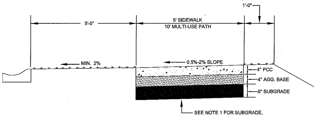
SIDEWALK / MULTI-USE PATH WITH GREEN SPACE NOT TO SCALE
