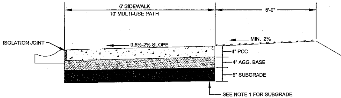
SIDEWALK / MULTI-USE PATH AT BACK OF CURB NOT TO SCALE
